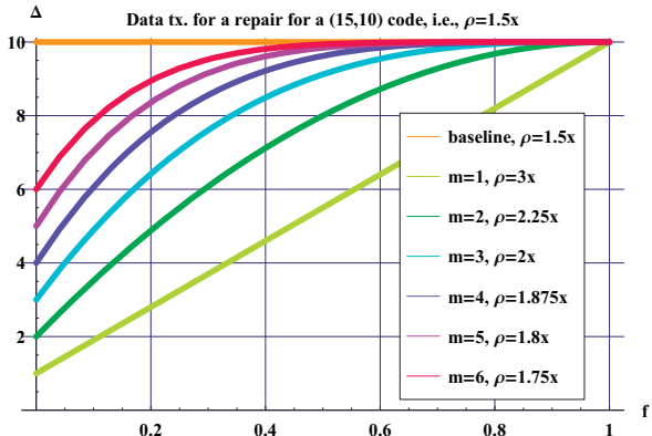
Figure 2: Data transfer for one repair
